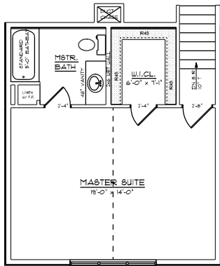
BONUS FLOOR PLAN 440 SQ. FT.
